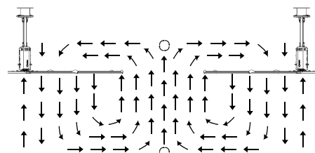
Air flow with multiple fans
