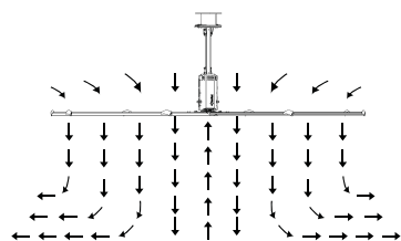
Air flow in an open area
